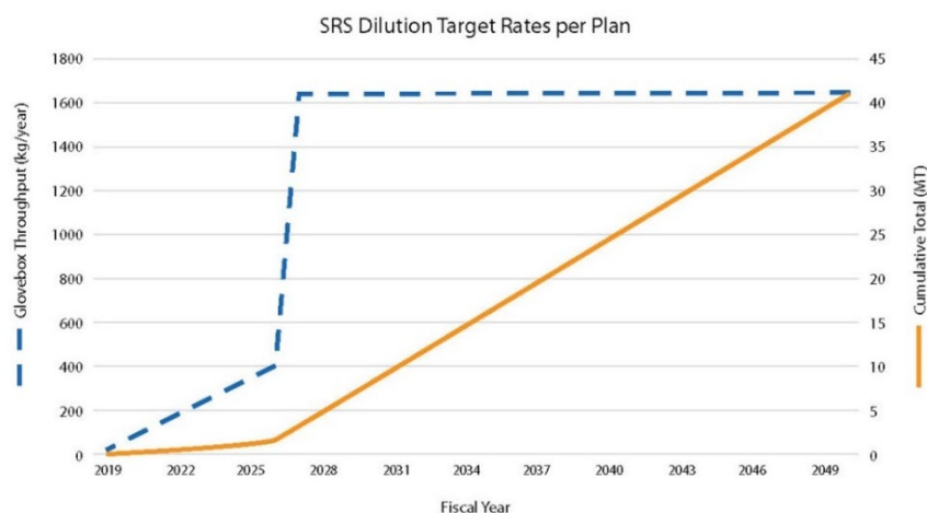
FIGURE 3-7 Graph of the dilution rates and cumulative production of diluted surplus plutonium as a function of time.
