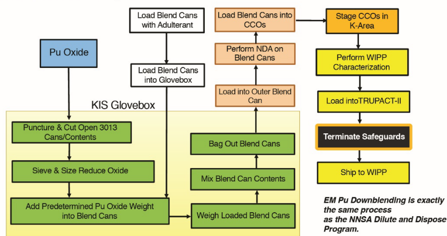
FIGURE 3-3 Process steps for dilution of the 6 MT of surplus non-pit plutonium material that is managed by DOE-EM. As noted in the figure, DOE-NNSA’s processing steps are the same as shown. A similar flowchart outlining the same steps is in DOE-NNSA’s dilute and dispose planning documents and can be seen in the committee’s Interim Report as Figure 2-3a. Safeguards are terminated when the packaged and characterized DSP-TRU waste is placed into the TRUPACT-II shipping container. The termination of safeguards step has been added to this flowchart based on information the committee was provided by DOE-NNSA. “Termination of safeguards” means the requirements for material control and accountability are removed but it does not mean that security is terminated (see Box 2-3 for more details). KIS = K Interim Surveillance. SOURCE: Modified from Maxted, 2019, slide 8.
