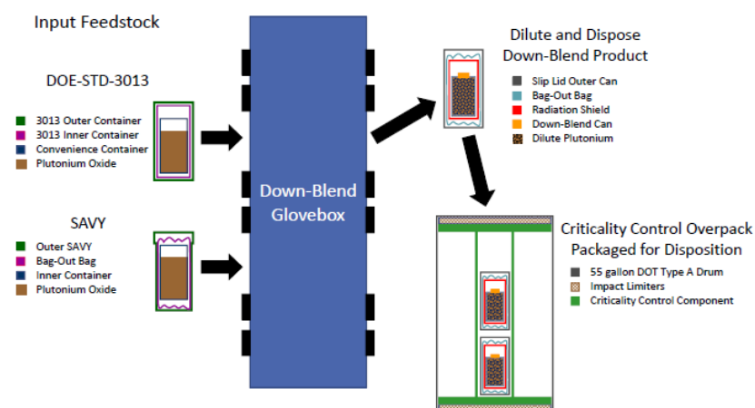
FIGURE 3-4 A schematic showing the different surplus plutonium containers that are used in the process of dilution. The 3013 and SAVY containers store plutonium oxide from LANL. The 3013 has welded closures, the SAVY container has a twisted closure and has been proposed by the dilute and dispose program for processing efficiency gains. The surplus plutonium oxide is diluted and mixed within an inner can which is bagged outside of the downblend glovebox and then placed into an outer can (KIS Glovebox in Figure 3-3). Two outer cans are placed into a single criticality control container (CCC, green outline and arrow), which is positioned inside of the criticality control overpack (CCO). NOTE: The figure refers to this as a Criticality Control Component ; the committee has seen both terms used, but criticality control container is used more frequently. SOURCE: Cantey and Robertson, 2019, slide 7. Image provided by the Department of Energy.
