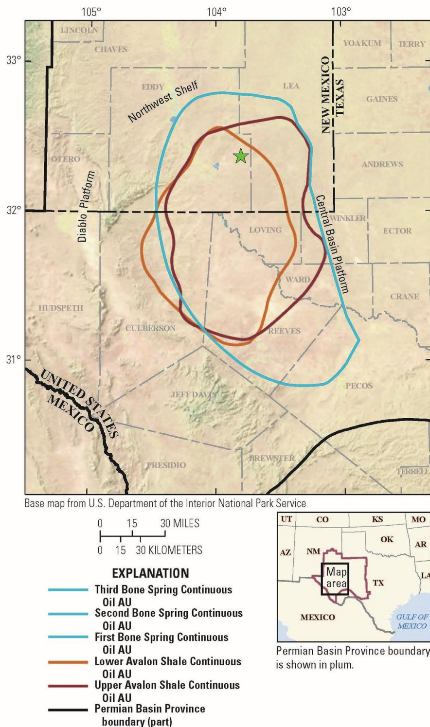
FIGURE 2-4 Oil-bearing shale formations in the Delaware Basin as recently identified by the U.S. Geological Survey. The Third, Second, and First Bone Spring Assessment Units (AUs) are overlapping and are shown by a single blue line. An orange line indicates the Lower Avalon Shale formation, and the maroon line indicates the Upper Avalon Shale formation. A green star (latitude 32.37, longitude 103.79) indicates the 4-mile-by-4-mile WIPP location. SOURCES: Gaswirth et al., 2018; USGS, 2018.
