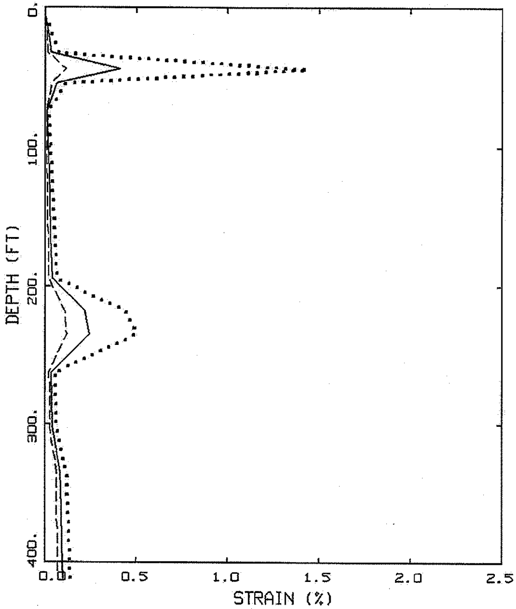
TA16: 10,000 YEAR, PGA ALL CASES, STRAINS (EYZ)
