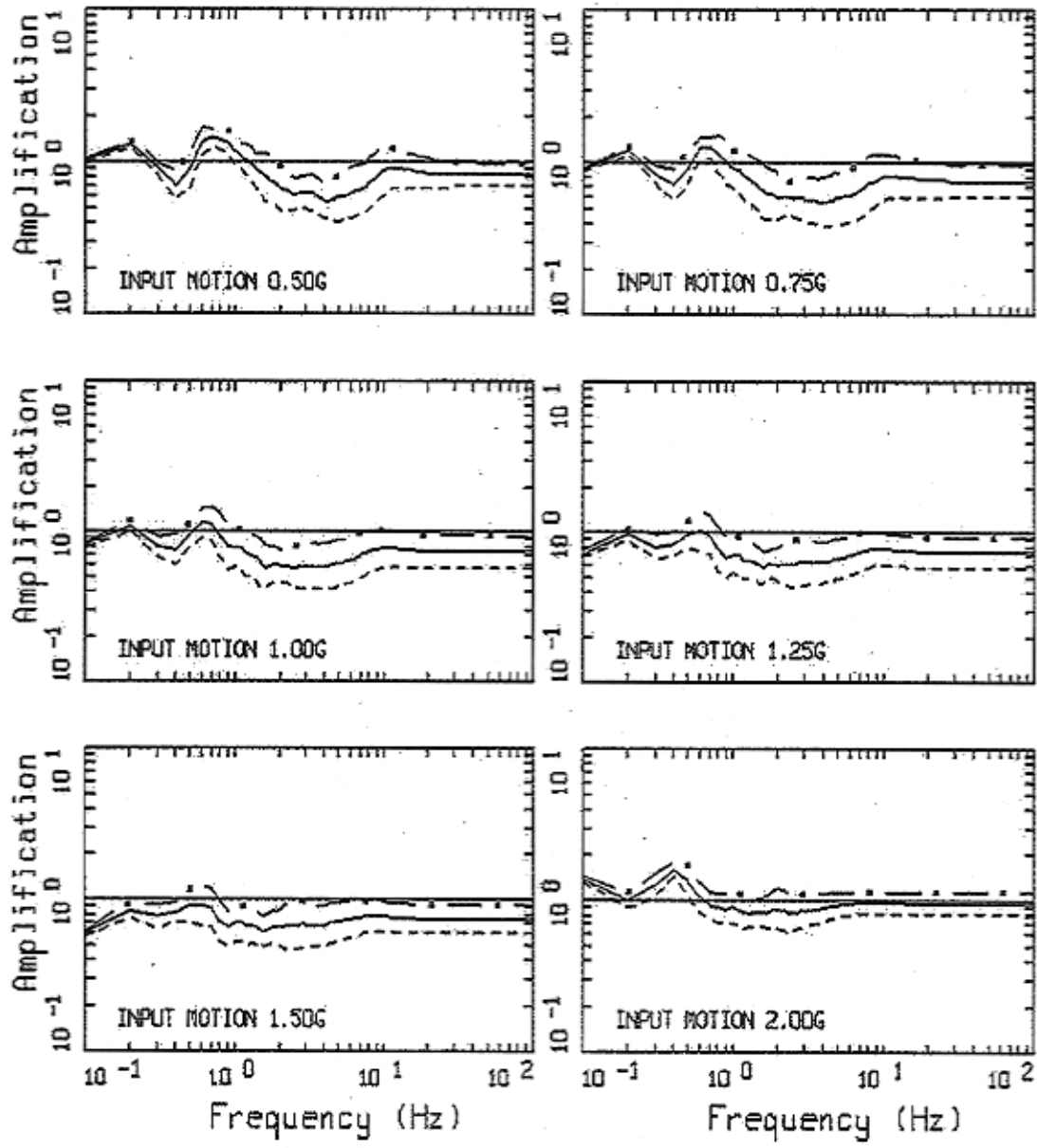
AMPLIFICATION, CMRR WNA: PAGE 2 OF 3 STOKE 04 UNADJUSTED, PROFILE A, HORIZ.
