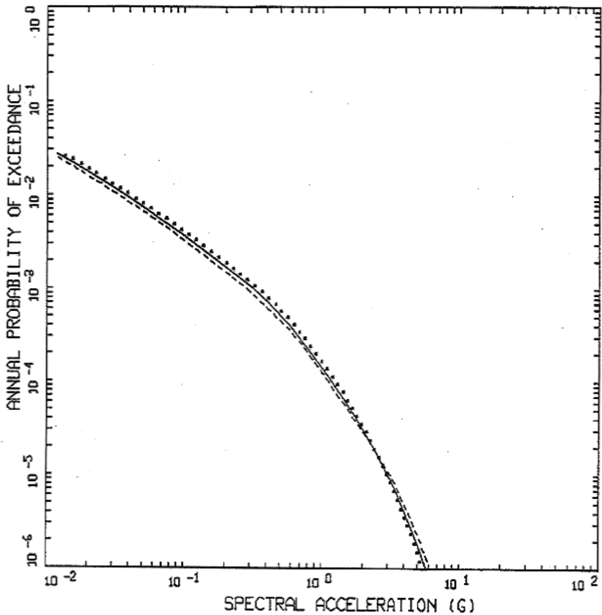
ALAMOS.05-VERTICAL (10/06) MEAN CURVES, PGA
