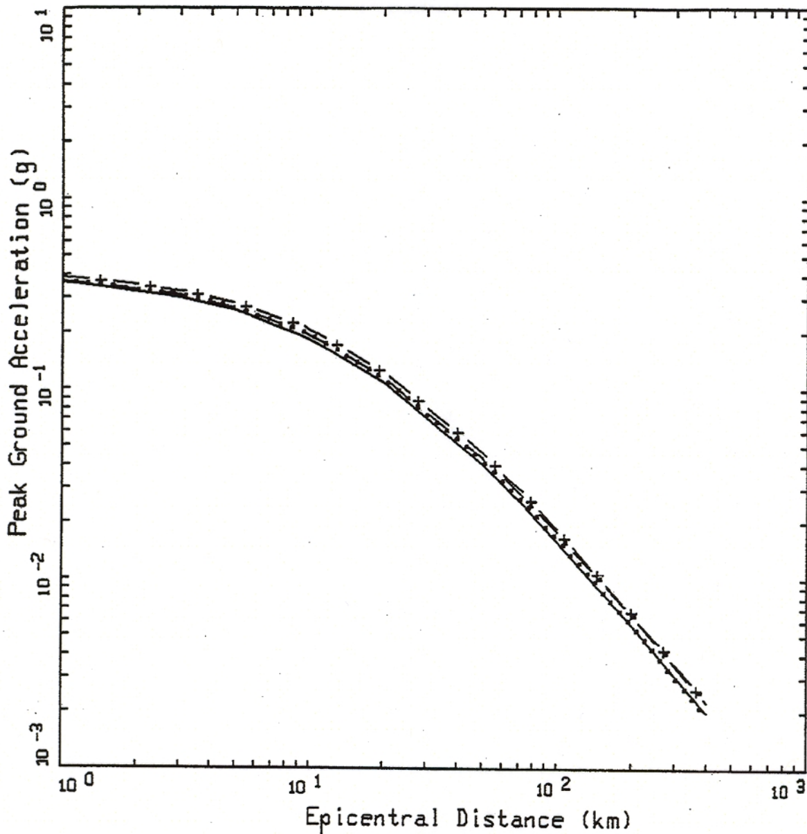
CMRR 1CVSD.M FOUR CASES (5/06) EPICENTRAL DIST, PGA
