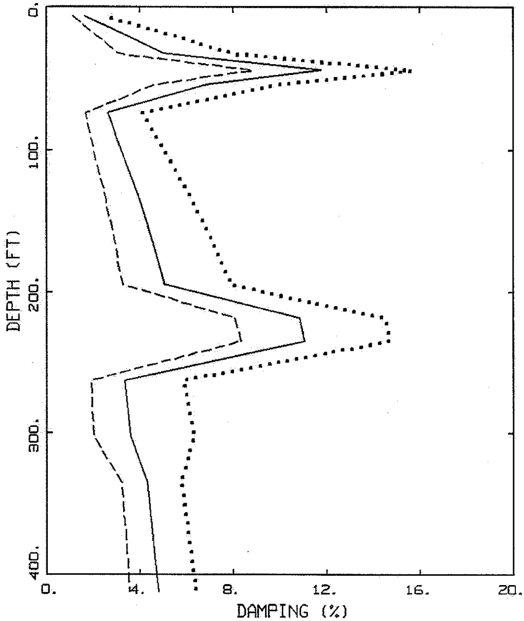
TA16: 10,000 YEAR, PGA ALL CASES, SHEAR WAVE DAMPING
