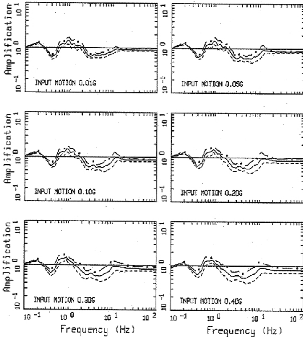
AMPLIFICATION, CMRR WNA: PAGE 1 OF 3 STOKO 04 UNADJUSTED, PROFILE A, HORIZ.
