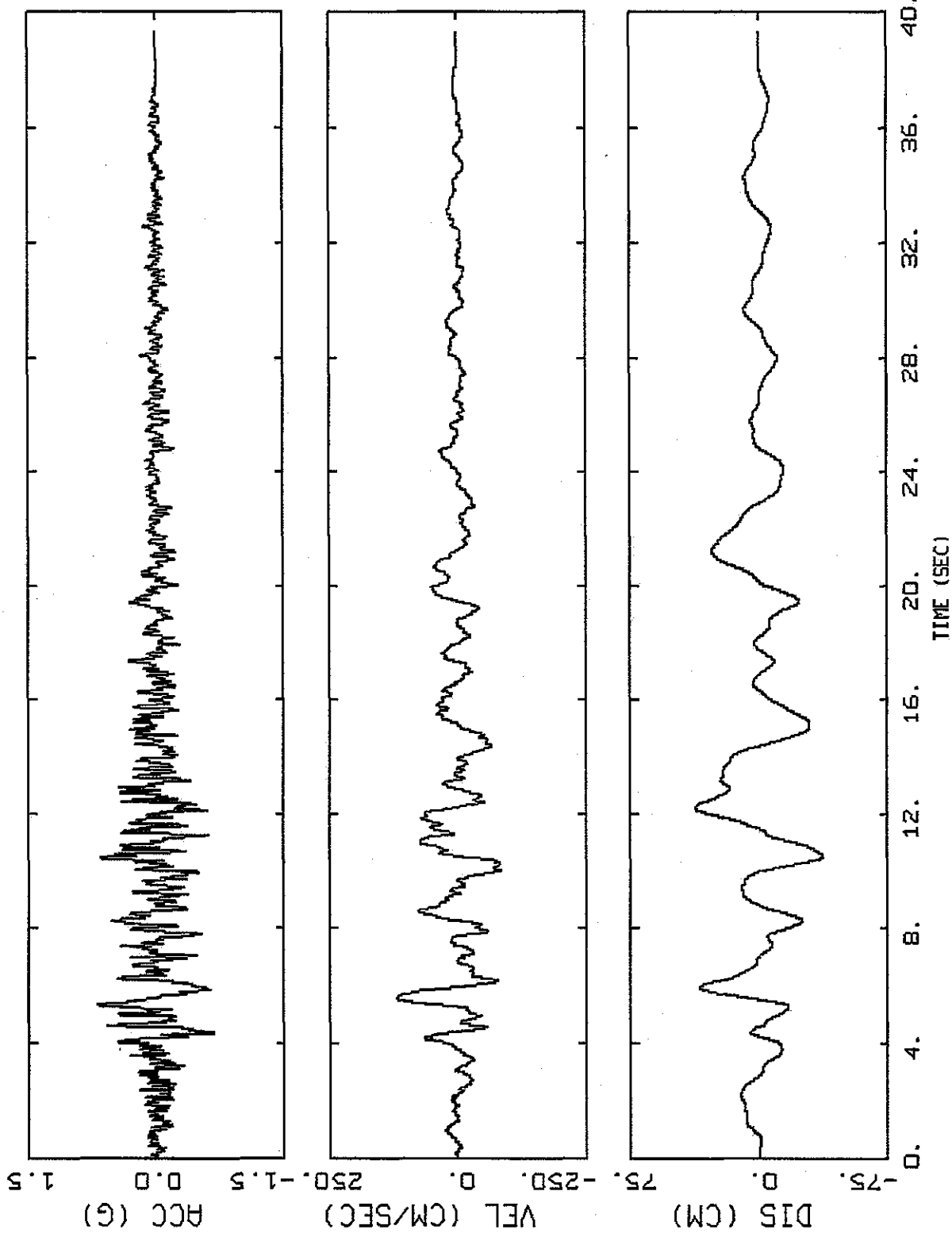
SITE-WIDE, SDC 4, 2% 50 YR, HORIZONTAL 1 BASELINE CORRECTED
