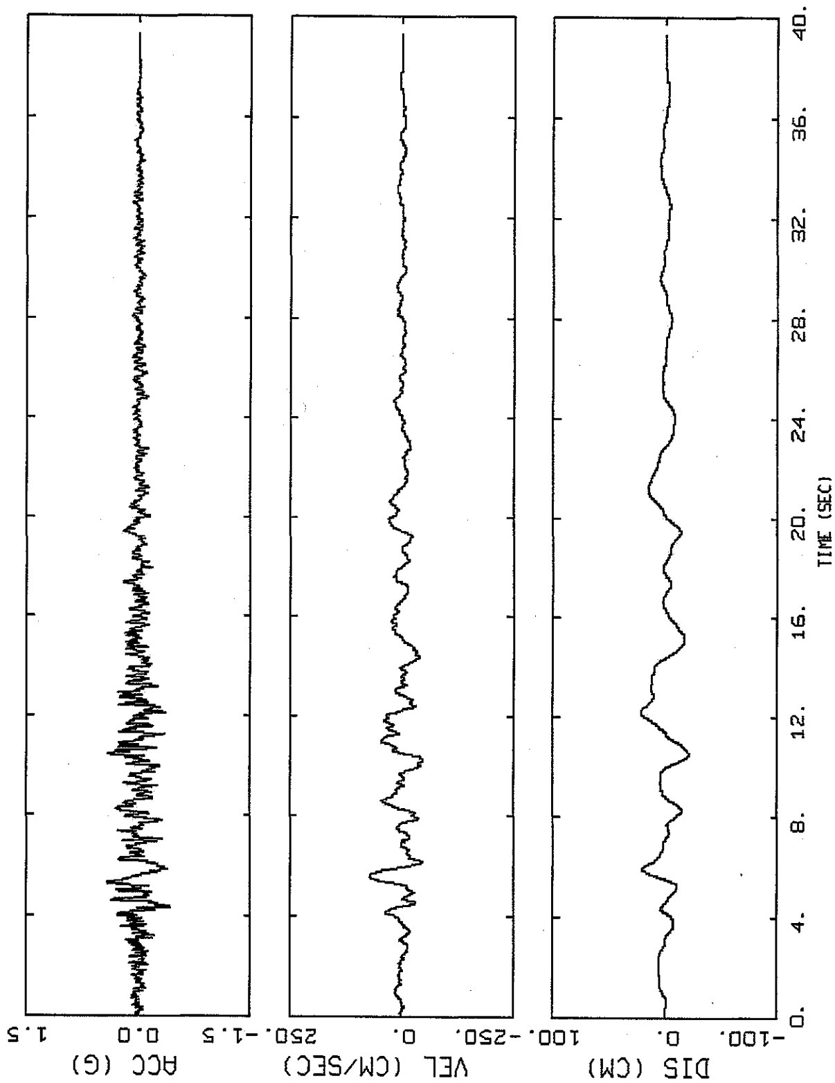
CMRR/TA-55 ENV., SDC 3, 2% 50 YR, HORIZONTAL 1 BASELINE CORRECTED
