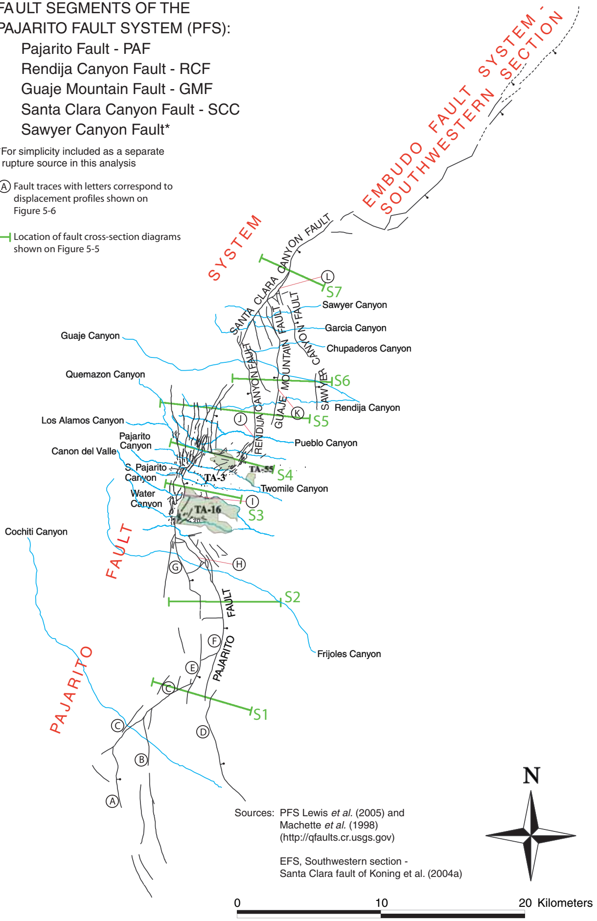
MAP OF THE PAJARITO FAULT SYSTEM AND ADJACENT SOUTHWESTERN SECTION OF THE EMBUDO FAULT SYSTEM
