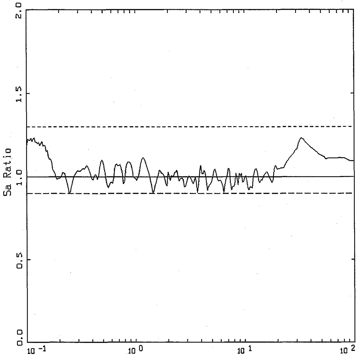
Frequency (Hz) DACITE, SDC 4, 2% 50 YR, HORIZONTAL 2 SPECTRAL RATIO: MATCH/TARGET
